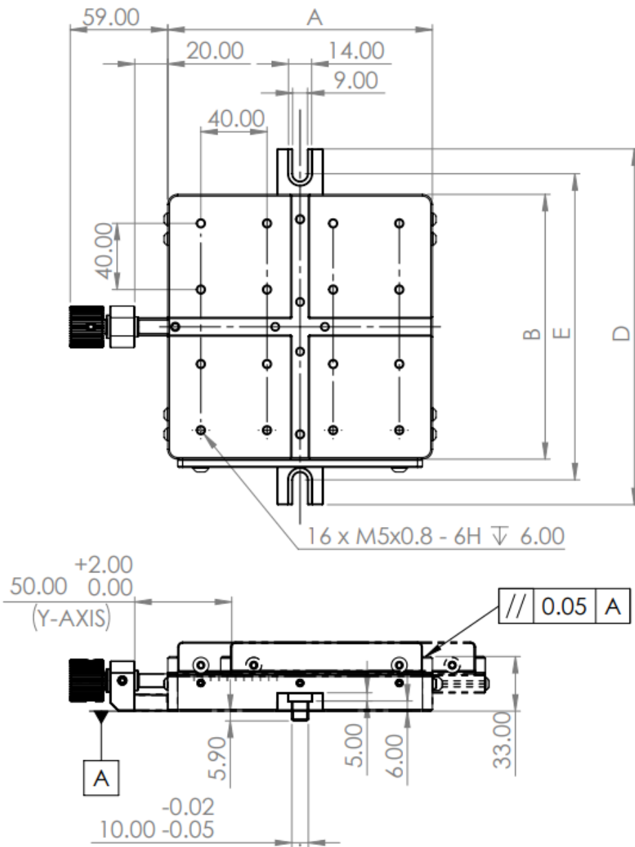
Dimension: Three Variants
