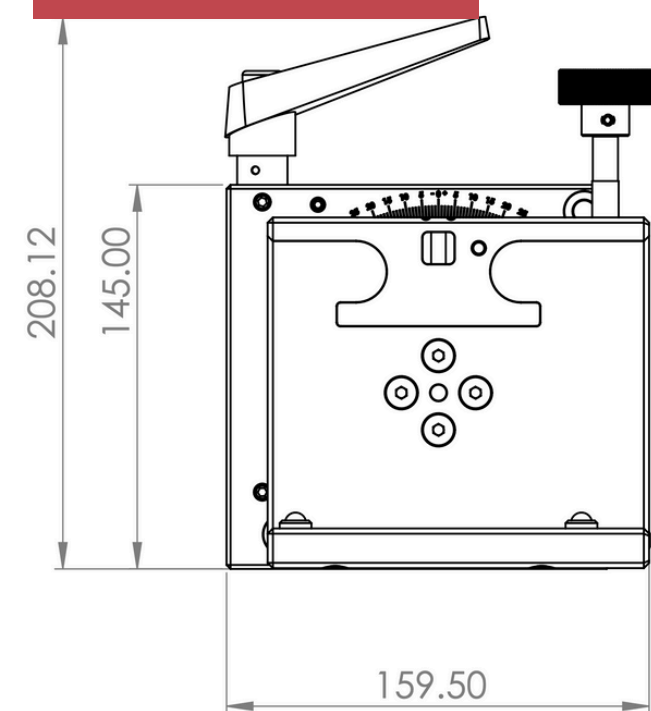
1253017 - MANUAL TILTING UNIT
