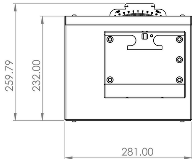
1252003 - MOTORISED TILTING UNIT
